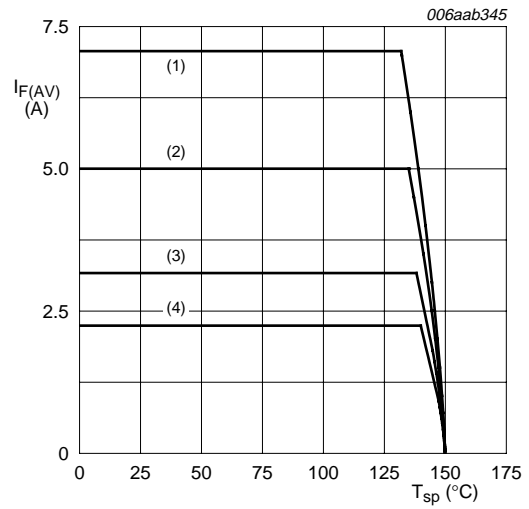
T_j = 150\text{ }^\circ\text{C} (1) \delta = 1 ; DC (2) \delta = 0.5 ; f = 20 kHz (3) \delta = 0.2 ; f = 20 kHz (4) \delta = 0.1 ; f = 20 kHz
