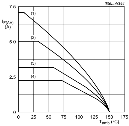
Ceramic PCB, Al_2O_3 , standard footprint T_j = 150\text{ }^\circ\text{C} (1) \delta = 1 ; DC (2) \delta = 0.5 ; f = 20 kHz (3) \delta = 0.2 ; f = 20 kHz (4) \delta = 0.1 ; f = 20 kHz
