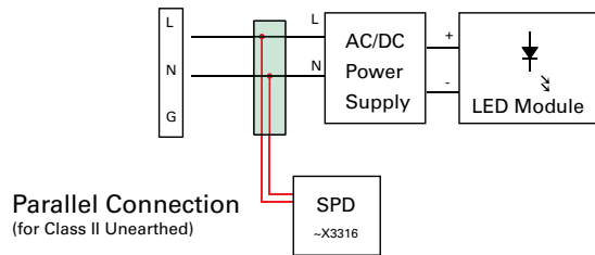
Parallel Connection
