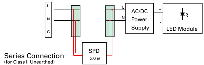
Series Connection
