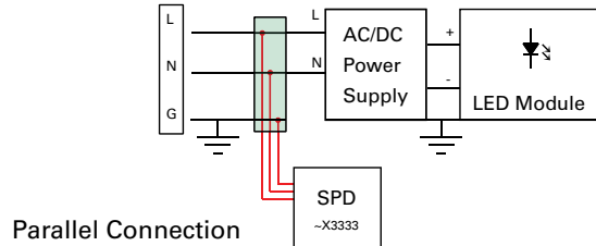
Parallel Connection
