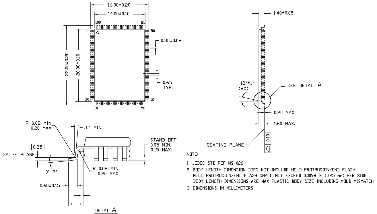
Figure 9. 100-pin TQFP (14 × 20 × 1.4 mm) A100RA Package Outline, 51-85050
