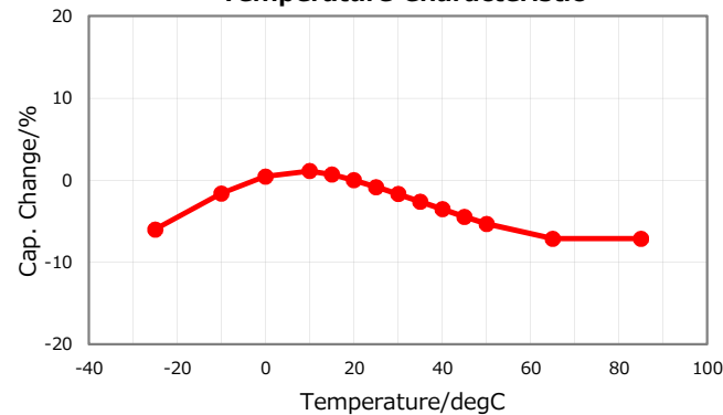
Temperature Characteristic
