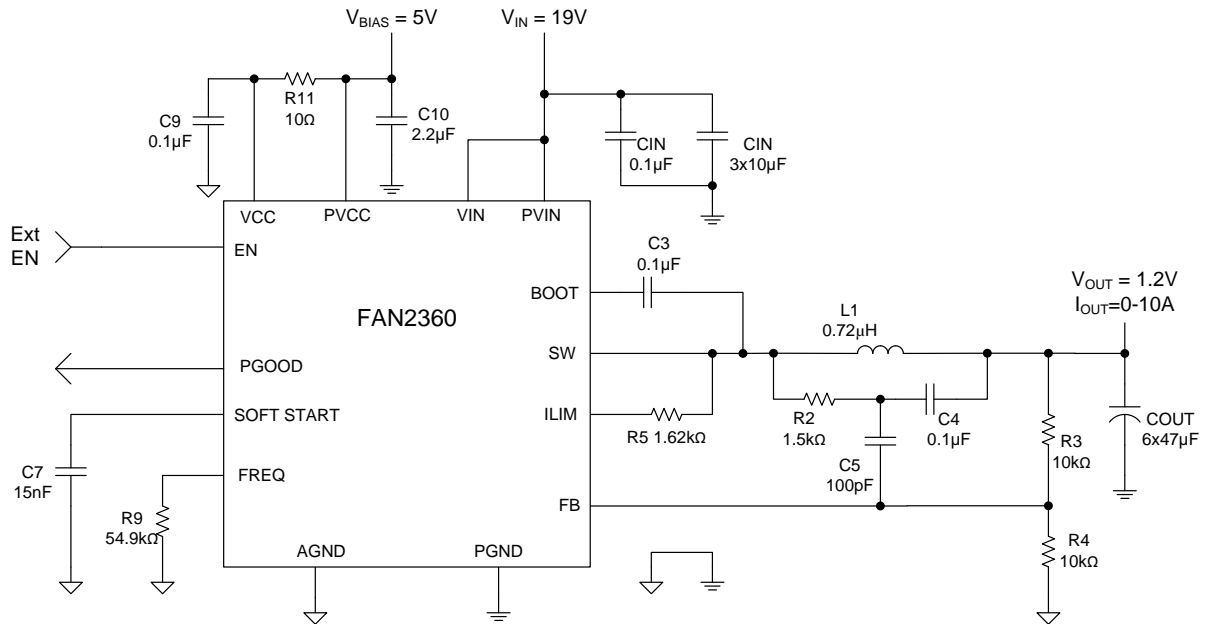
Figure 1. Typical Application
