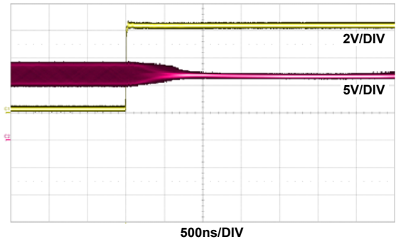
FIGURE 40. POWER-DOWN TIME
