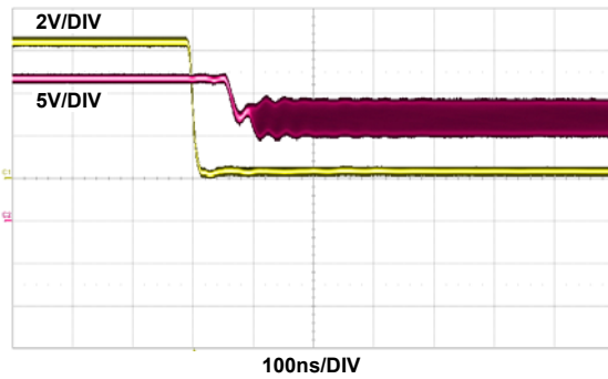
FIGURE 39. POWER-UP TIME
