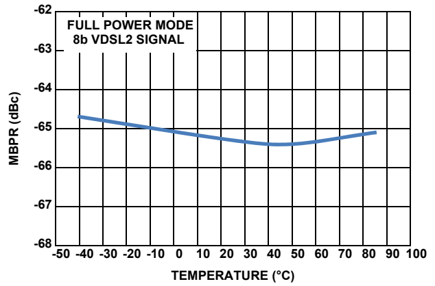
FIGURE 45. 8b MBPR vs TEMPERATURE
