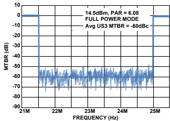
FIGURE 32. VDSL2 30a PROFILE MTBR US3
