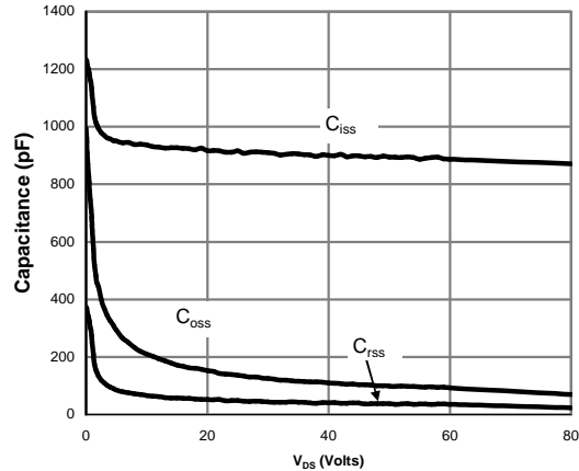
Figure 8: Capacitance Characteristics
