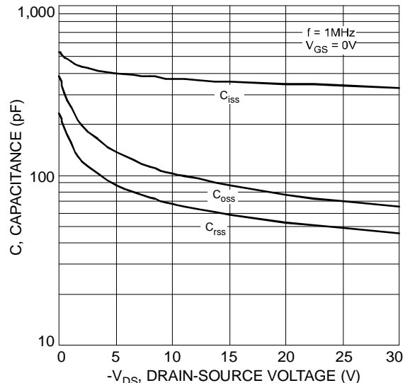
Fig. 15 Typical Capacitance
