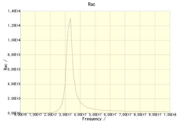
CLF10040T-100M-CA
