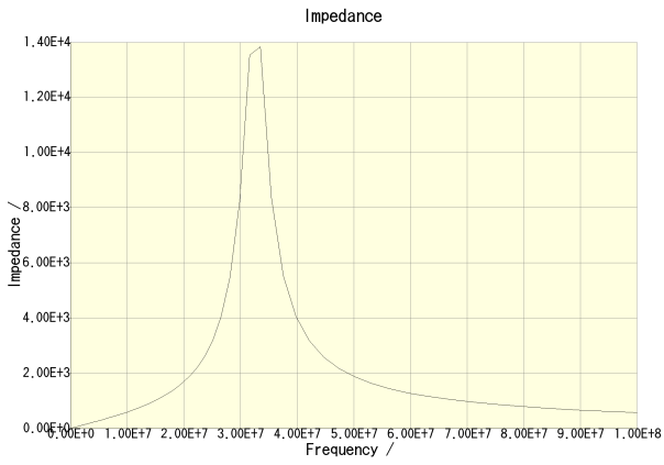
CLF10040T-100M-CA
