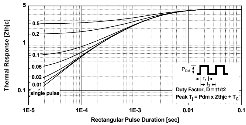
Figure 23. Transient Thermal Impedance of FRD
